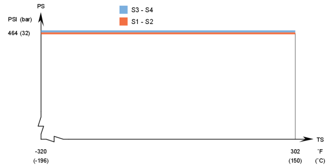
CB18 – PED approval pressure/temperature graph
