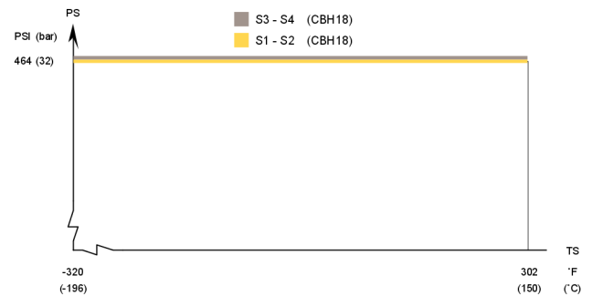
CBH18 – UL/CRN approval pressure/temperature graph
